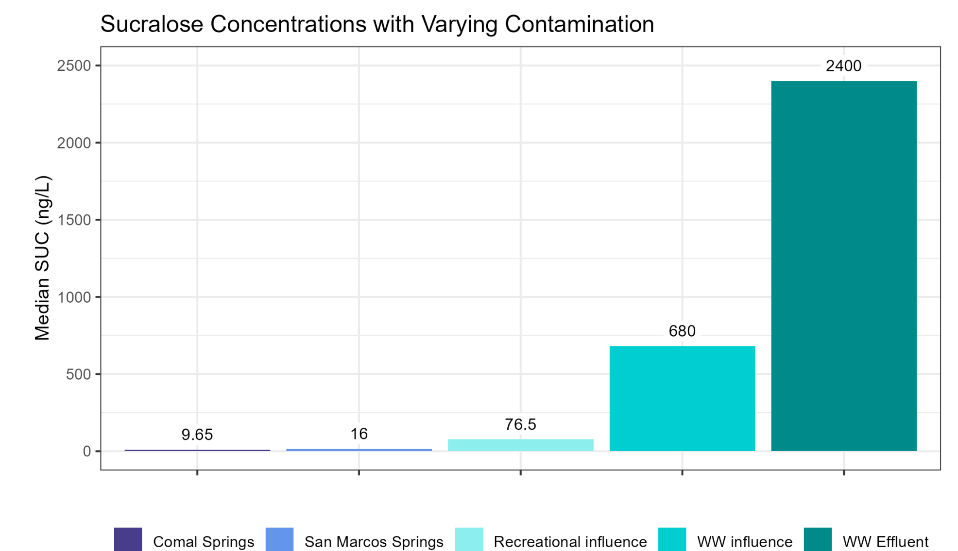
Figure 3: Sucralose concentrations in the Edwards Aquifer springs groundwater compared to average U.S. surface waters with recreational influence 1 , surface waters with wastewater influence 2 , and wastewater effluent 3
